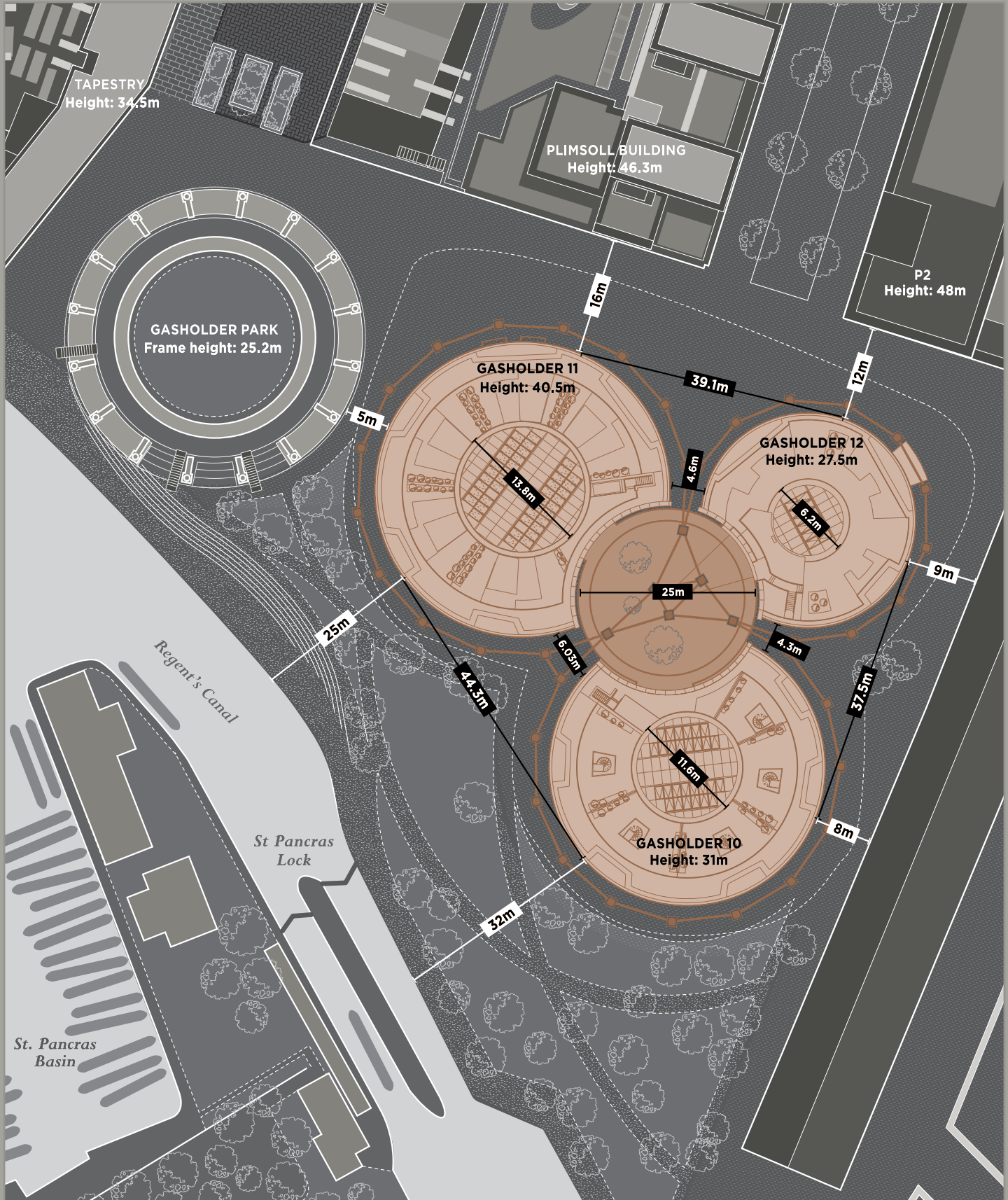
Plan illustrating approximate distances to, and heights of, neighbouring buildings Gasholders— King's Cross, London NIC
